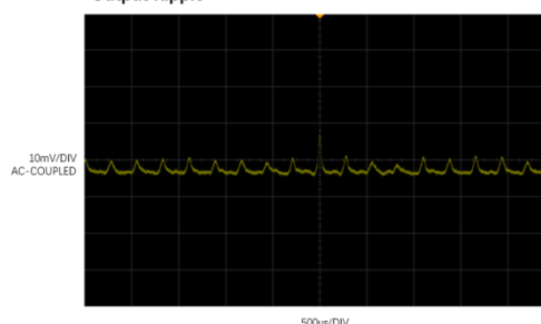
Output Ripple
