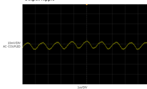
Output Ripple
