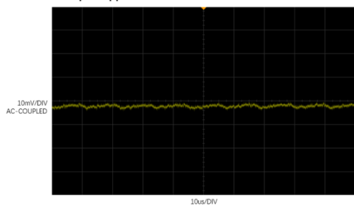
Output Ripple
