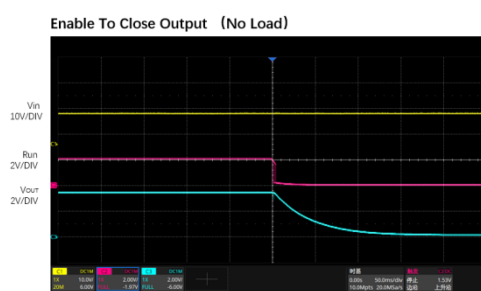
V_{in}=12V V_{out}=3.3V SOFT-START Capacitor=0.1uF Output Capacitor=47uF X2
