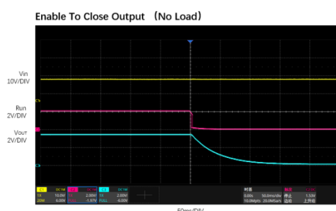
V_{in}=12V V_{out}=3.3V SOFT-START Capacitor=0.1uF Output Capacitor=47uF X2
