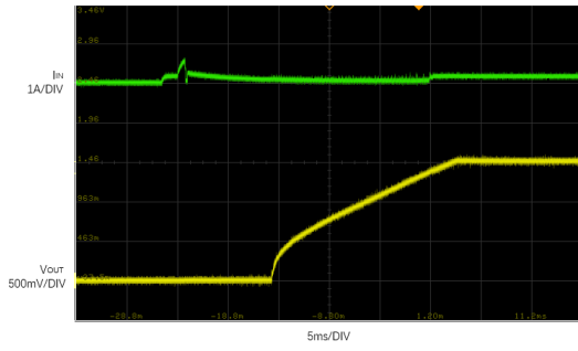
V_{in}=12V V_{out}=1.5V SOFT-START Capacitor=0.1uF Output Capacitor=47uf X2
