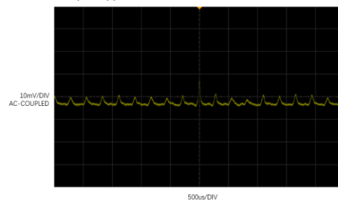
V_{in}=5V V_{out}=1.5V I_{load}=0A SOFT-START Capacitor=0.1uF Output Capacitor=47uf X2
